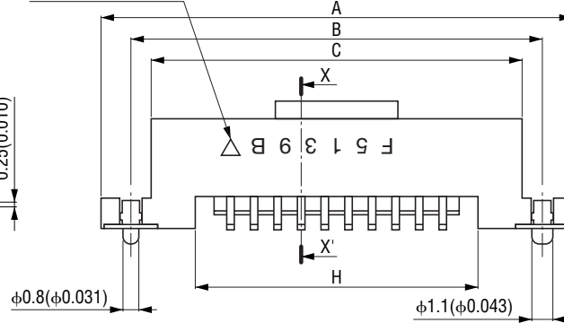
Polarity identification
