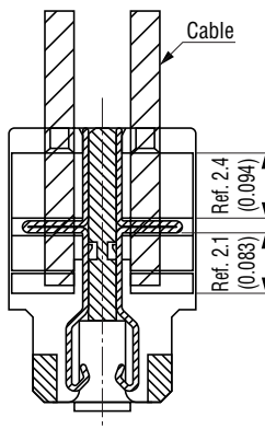
X-X' Cross Section
